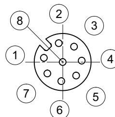
Pin Assignment
