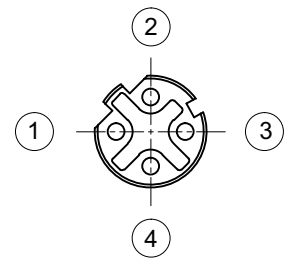
Pin Assignment
