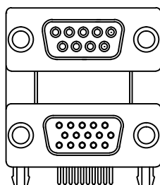
9P Female over 15P HD Female (DDPXR-E9S/E15S)
