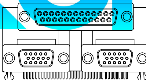
25P Female over 15P HD Female & 15P HD Female (DDPNXR-B25S/E15S+E15S)
