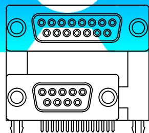
15P Female over 9P HD Female (DDPXR-A15S/E9SL)
