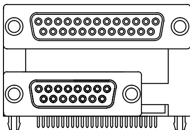
25P Female over 15P Female (DDPXR-C37S/A15SL)
