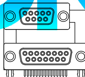
9P Female over 15P Female (DDPXR-E9SL/A15S)
