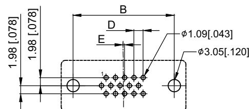
Recommended PCB Layout Male(Plug):Top View
