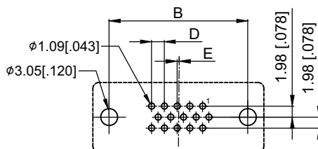
Recommended PCB Layout Female(Receptacle):Top View
