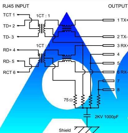
Magnetic Schematic
